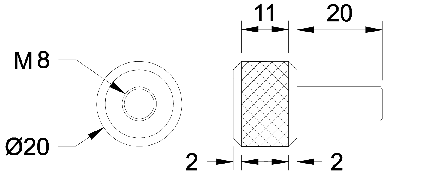
Part 6 lock component
